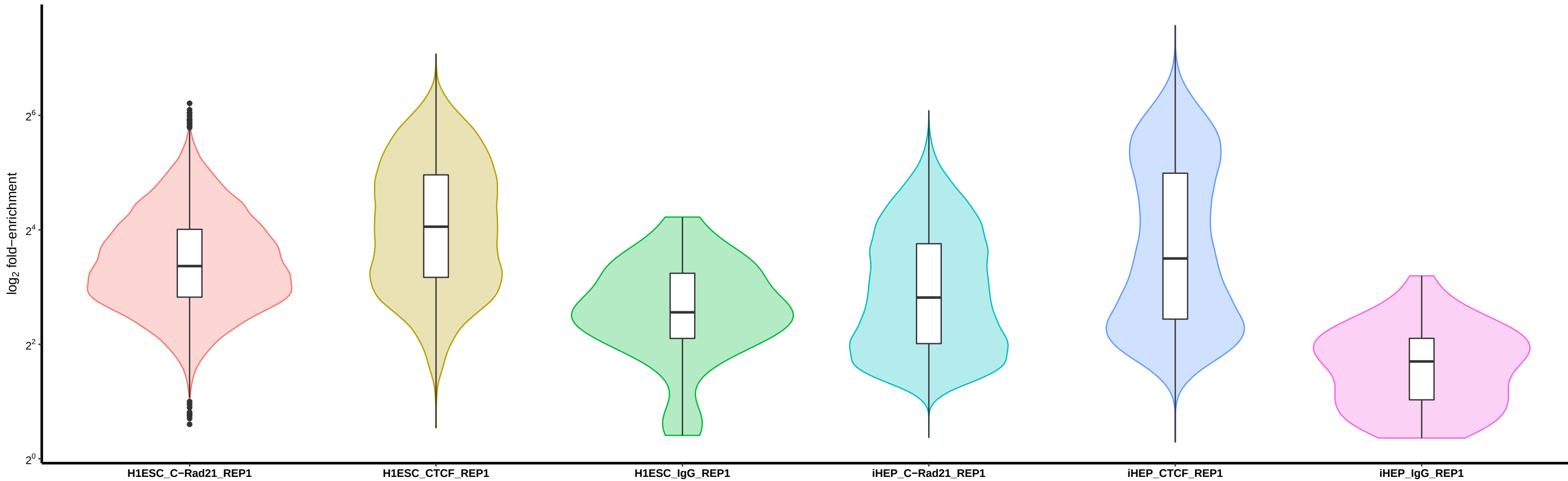
Fold-change distribution
