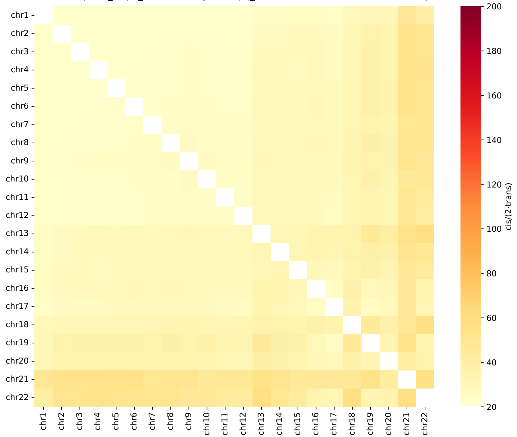
H9ESC_Nup155_DEp4_20241021.hg38.mapq_30.1000 • Chromosome territoriality
