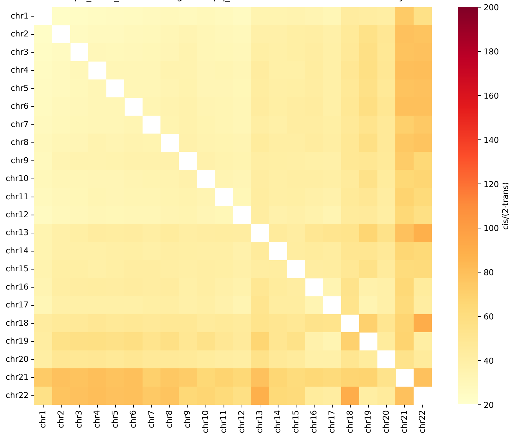
DEp6_HiC3_20240517.hg38.mapq_30.1000 • Chromosome territoriality
