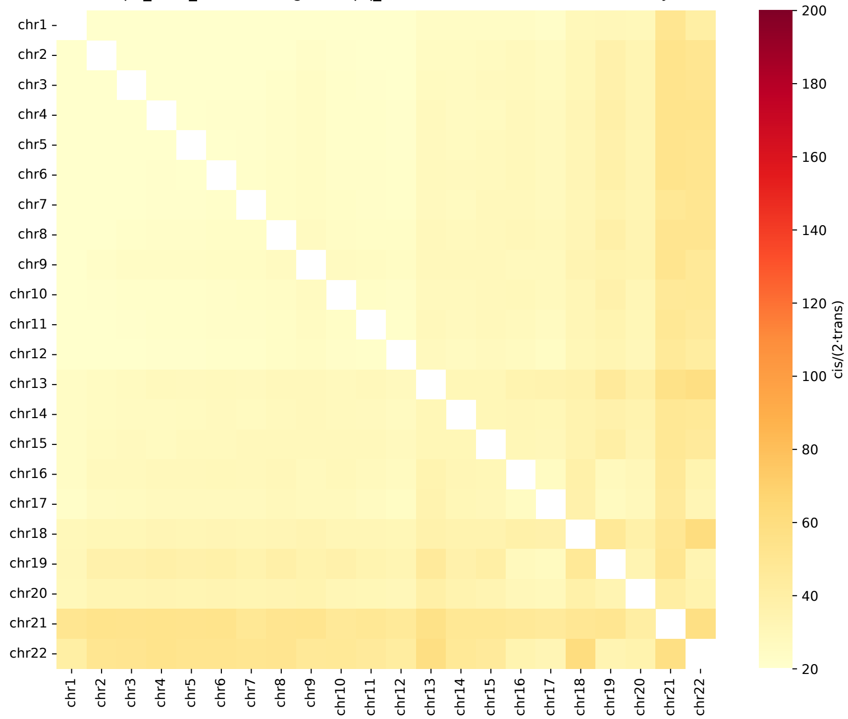
DEp3_HiC3_20240517.hg38.mapq_30.1000 • Chromosome territoriality
