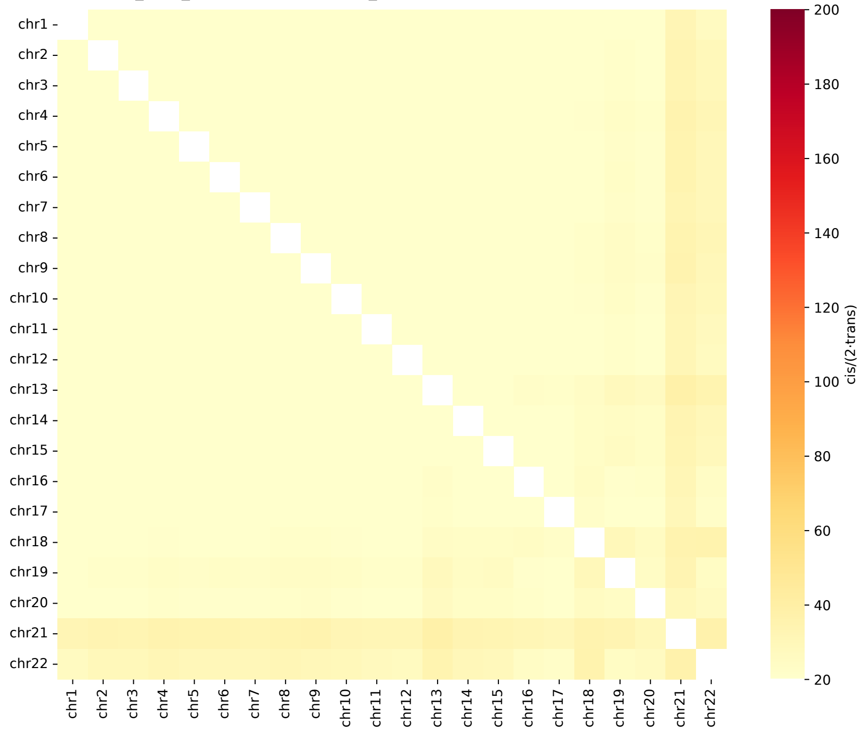
DE_HiC3_20240517.hg38.mapq_30.1000 • Chromosome territoriality
